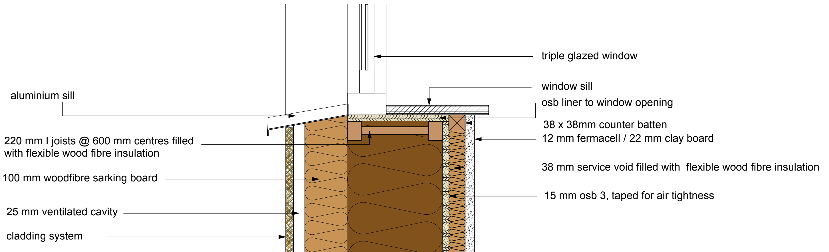
Suggested Window Reveal Detail in section - External Wood Fibre Insulation on Timber Frame - Timber Cladding
