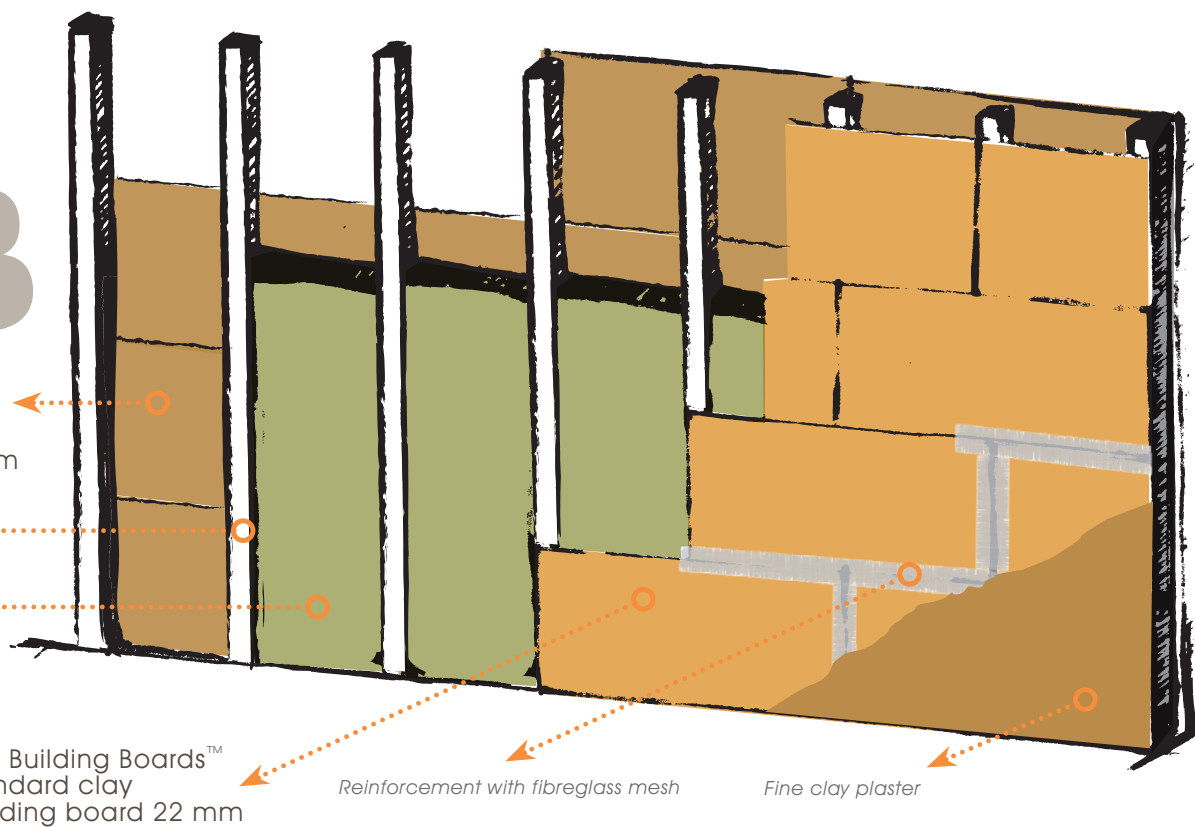
Natural, uniform radiation by the clay heating element/Climate clay building board
