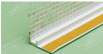
UdiREINFORCEMENT® Render Edging Strip INSIDE (D 10)
